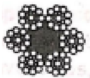
6 X 19 SEALE B
